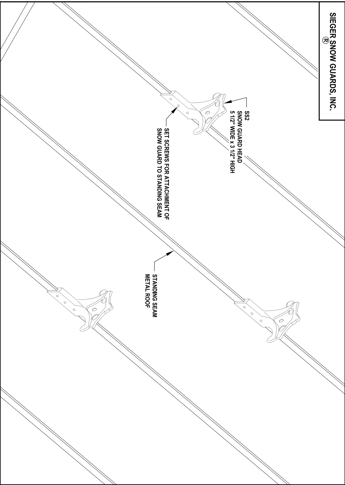
TYPICAL SS2 INSTALLATION DIAGRAM
