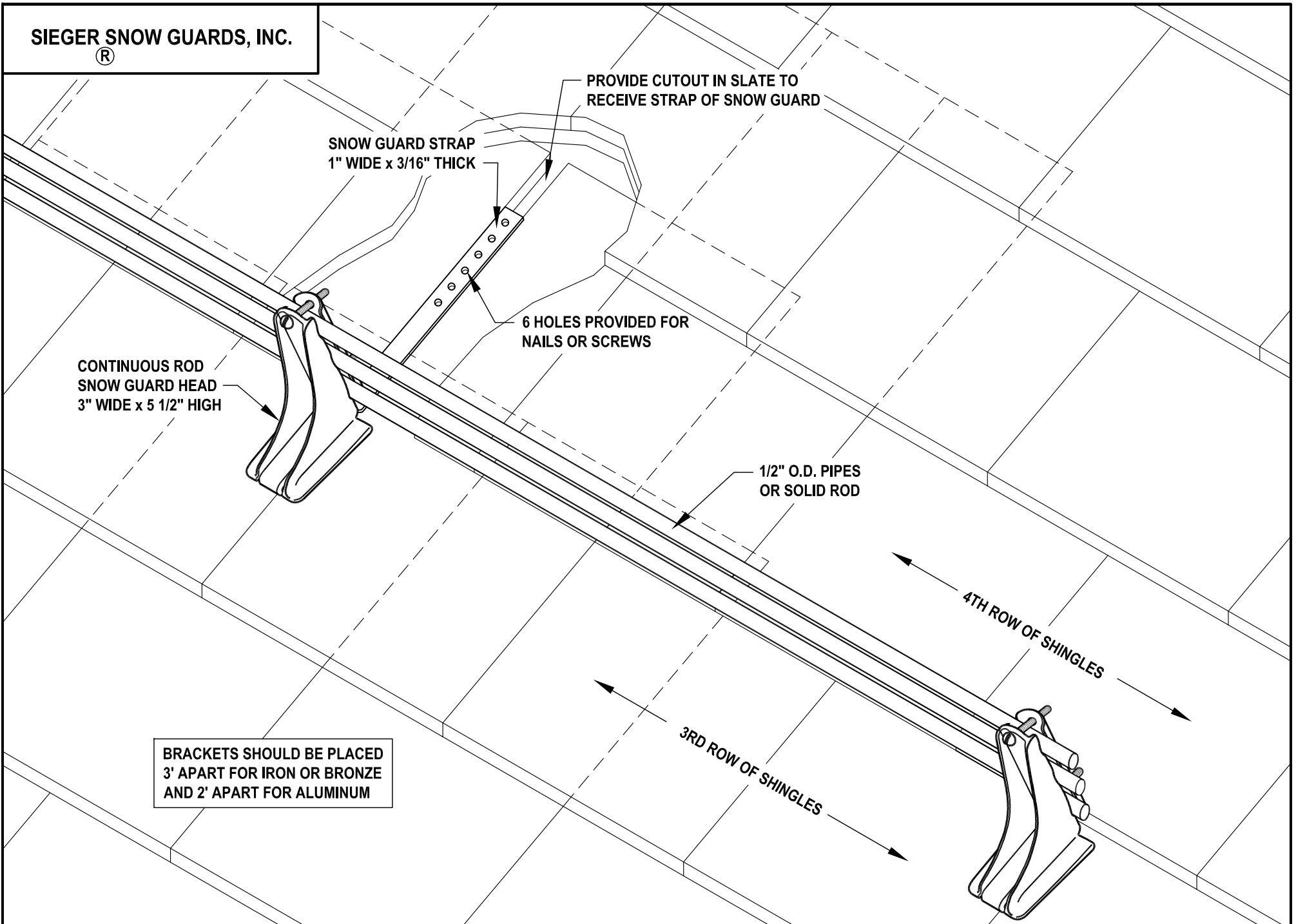
TYPICAL CONTINUOUS ROD INSTALLATION DIAGRAM
